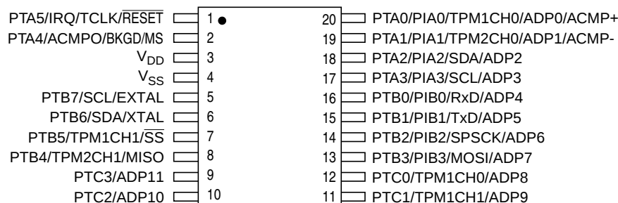
Figure 2-2. 20-Pin PDIP and TSSOP
