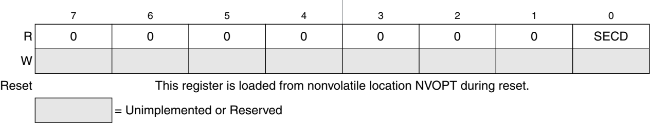
Figure 4-3. Flash Options Register (FOPT)
