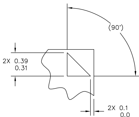
DETAIL T
